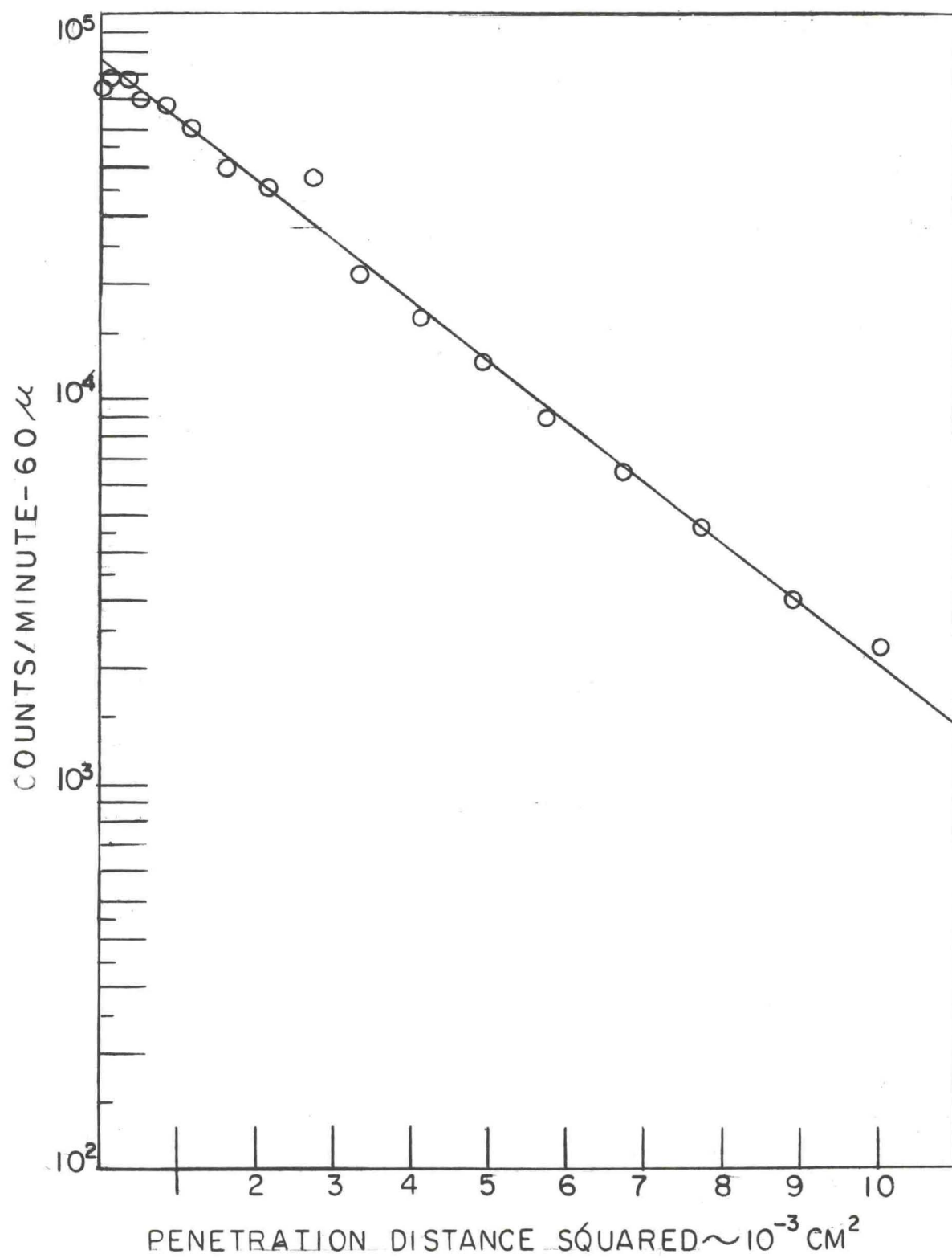
Figure 5. Solute Penetration Curve, Sample No. 68-- Annealed at 24 kb. pressure and 763°K for 3.18 \times 10^3 sec
